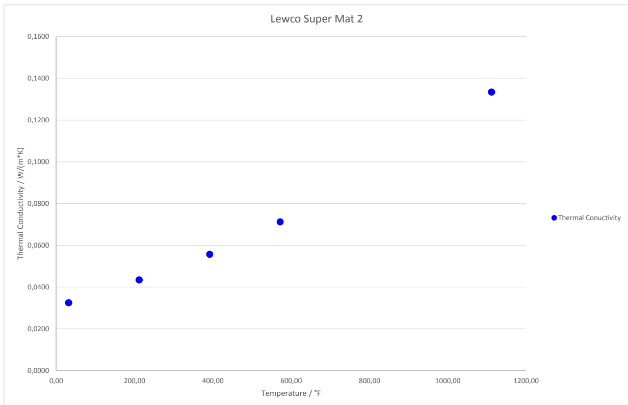
Figure 1: Thermal conductivity of Lewco Super Mat 2
